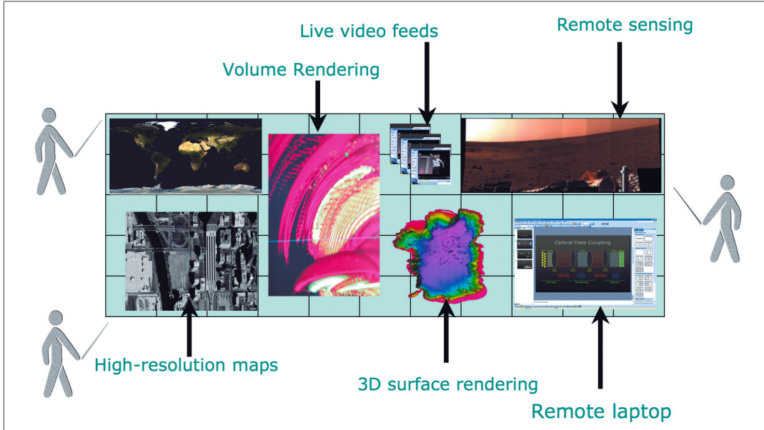
Figure 3.8: The Free Space Manager provides an intuitive interface for moving and resizing graphics on a tiled display. When a graphics window is moved from one portion of the screen to another, the Free Space Manager informs the remote rendering clusters of the new destination for the streamed pixels, giving the illusion of working on one continuous computer screen, even though each of their systems may be several thousand miles apart.
