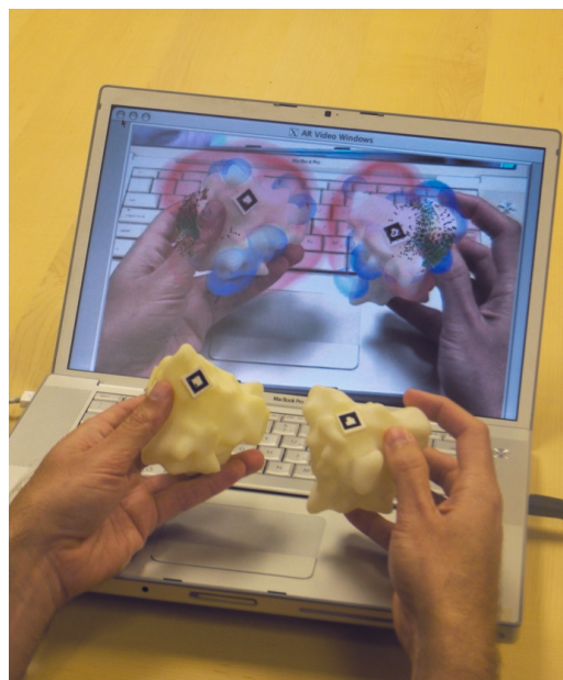
Figure 3.4: Computer augmentation of two subunits of the superoxide dismutase (SOD) dimer, which are tracked and manipulated independently. The electrostatic field is shown with small arrows that point along the local field vectors (they appear as small dots in this picture), and the potential is shown with volume rendered clouds, with positive in blue and negative in red.
